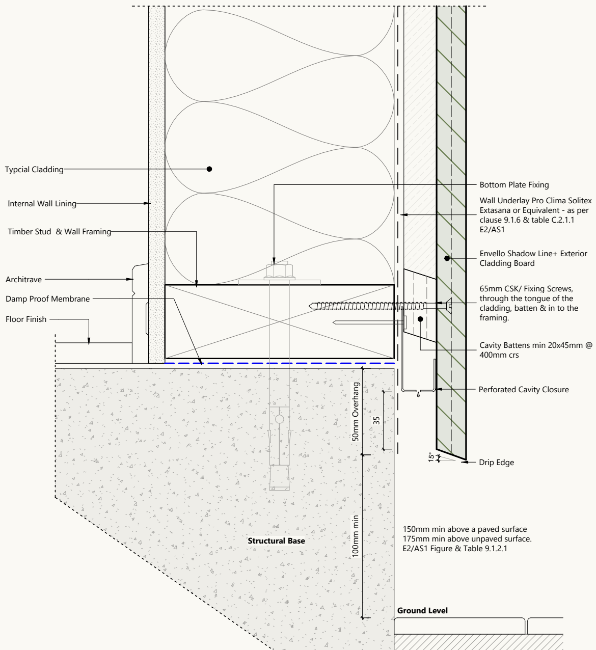
BASE TO WALL – GROUND LEVEL
