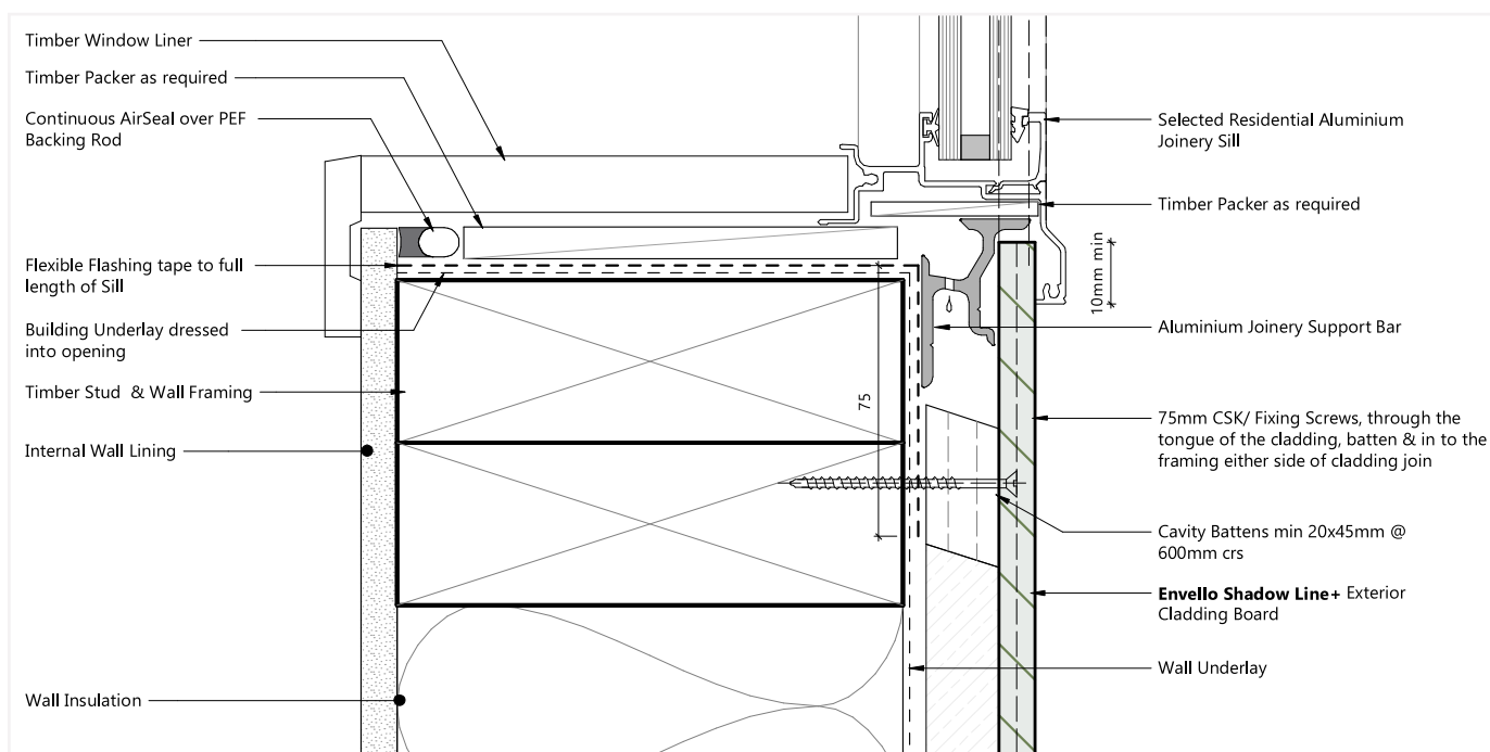
FIG.21 - WINDOW SILL
