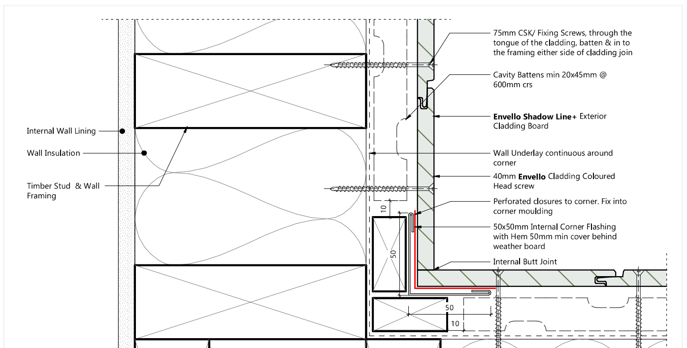
FIG.12 INTERNAL CORNER
