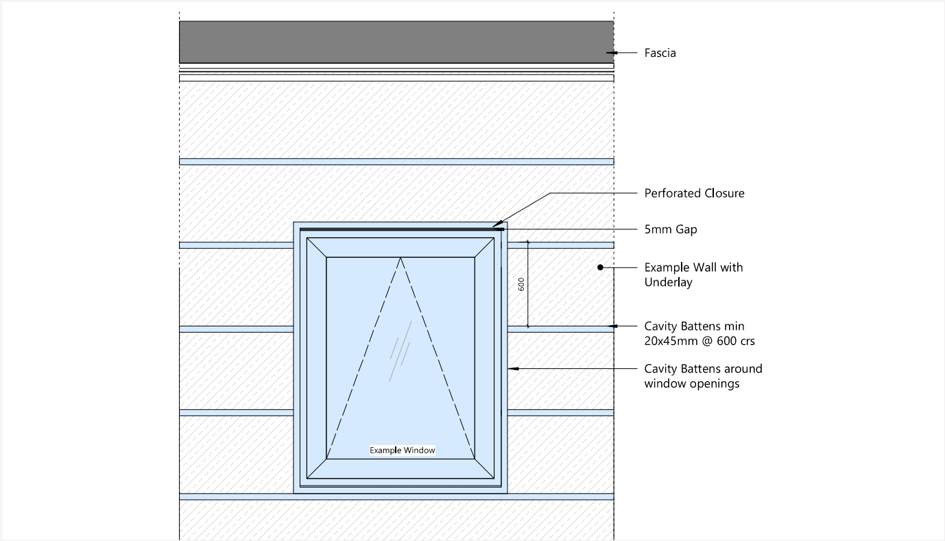
FIG.5 BATTEN LAYOUT AROUND AN OPENING
