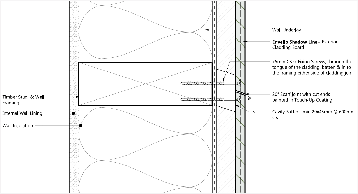
FIG.6 BOARD JOIN
