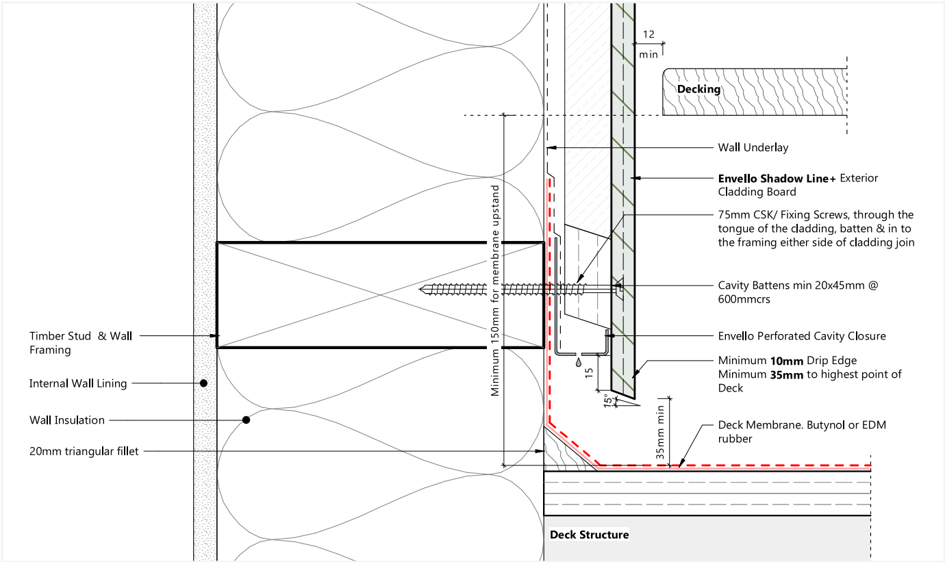
FIG.2 BASE TO DECK
