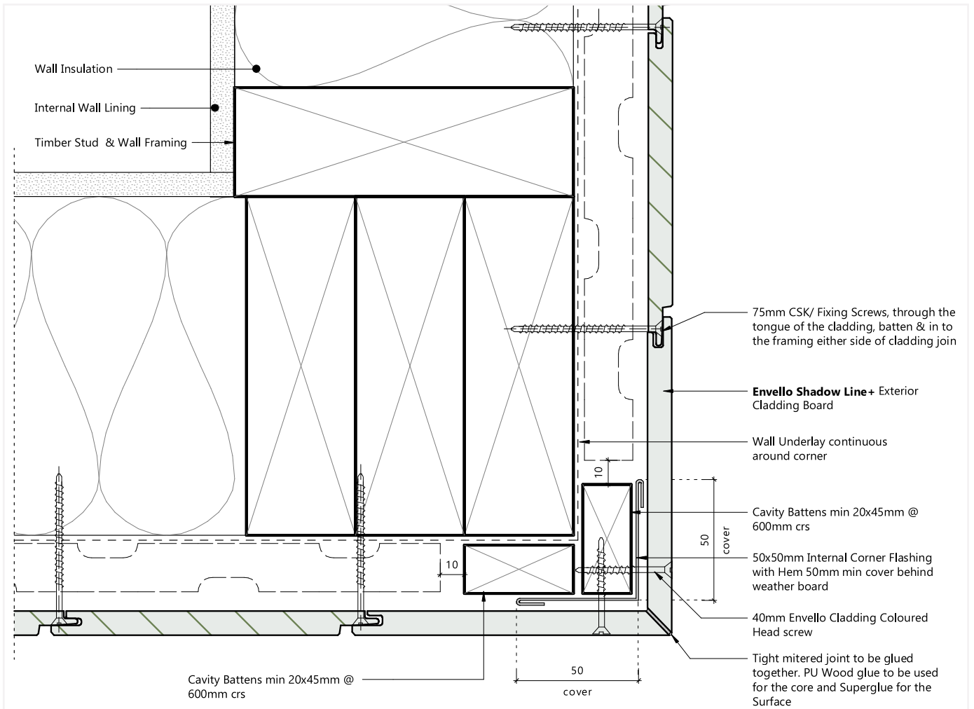
FIG.12 INTERNAL CORNER
