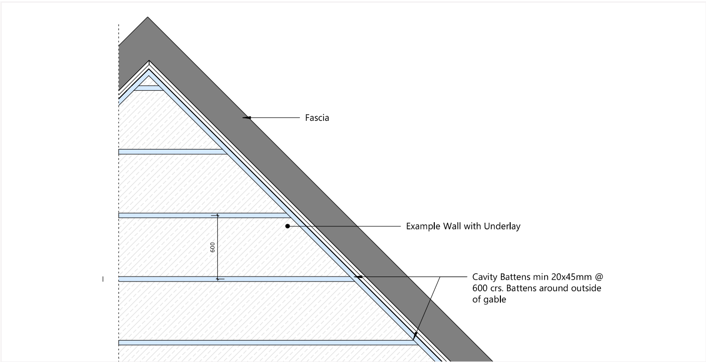
FIG.4 BATTEN LAYOUT AT A GABLE END
